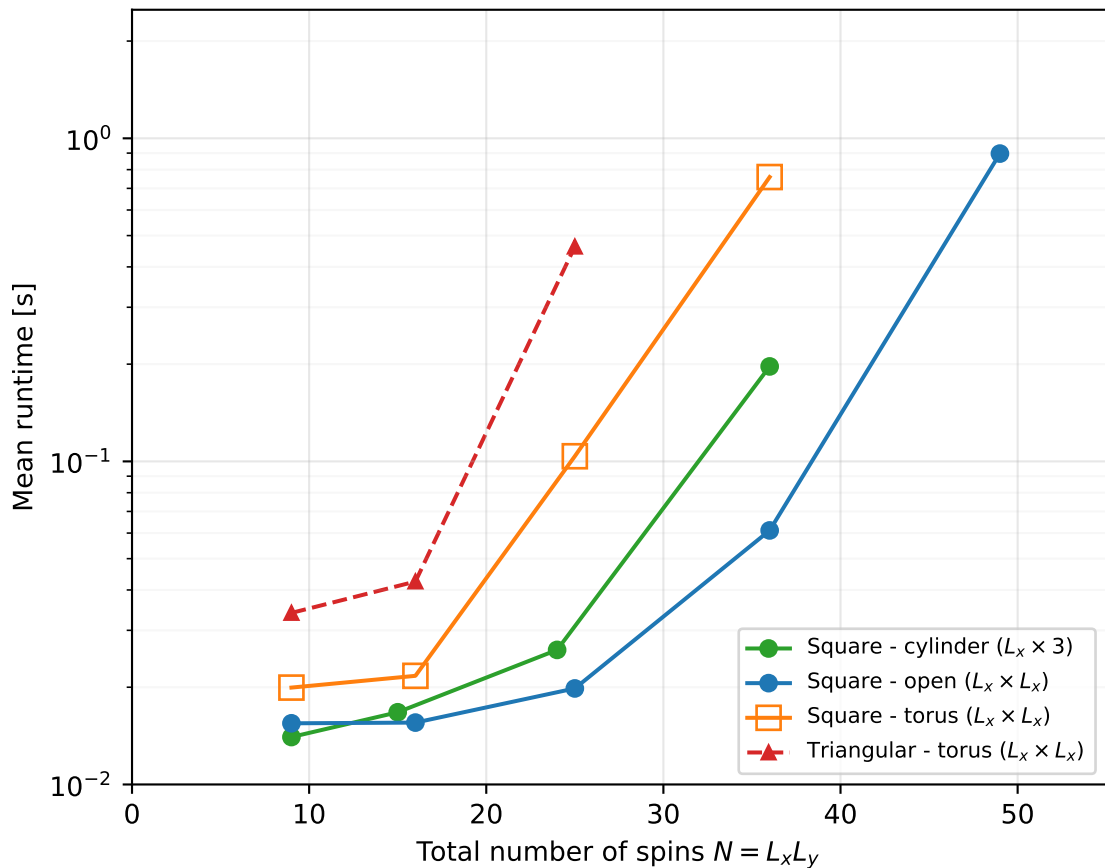
Runtime for Z using Cachet
